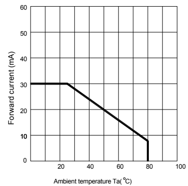
Fig.2 Forward current derating curve vs. ambient temperature
